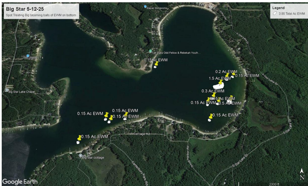
Figure 19. EWM Distribution in Big Star Lake (May 12, 2025).
