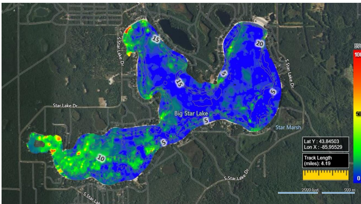
Figure 16: Biovolume map of Big Star Lake from the August 27th, 2025 scan.
